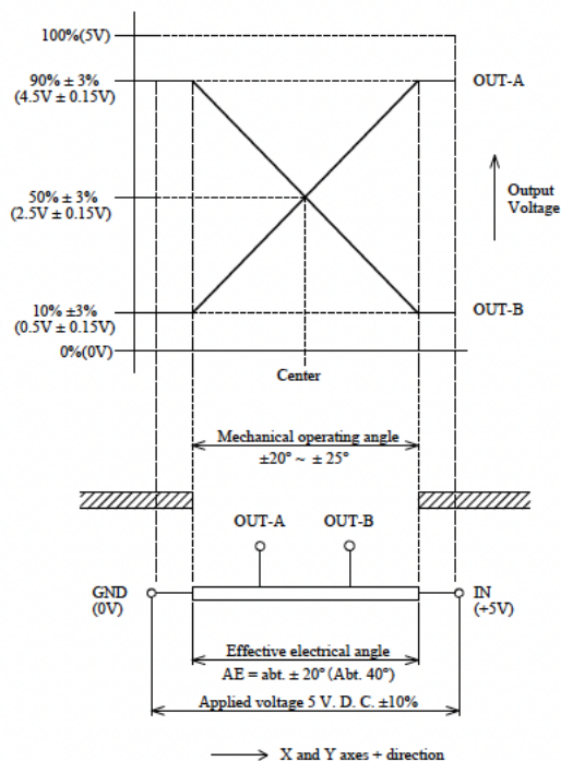
OUTPUT CHARACTERISTICS AND TERMINAL CONNECTION DIAGRAM FOR X AND Y AXES POT.
