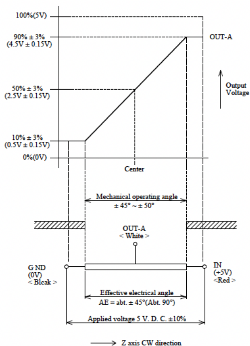
OUTPUT CHARACTERISTICS AND TERMINAL CONNECTION DIAGRAM FOR Z AXIS POT.
