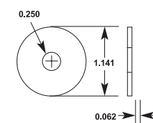
FIGURE 2. CONDUCTIVE WASHER
