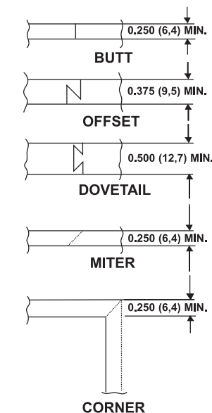
FIGURE 1. FOUR BASIC SPLICING TECHNIQUES
