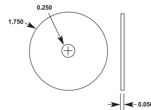
FIGURE 3. METAL COUPON
