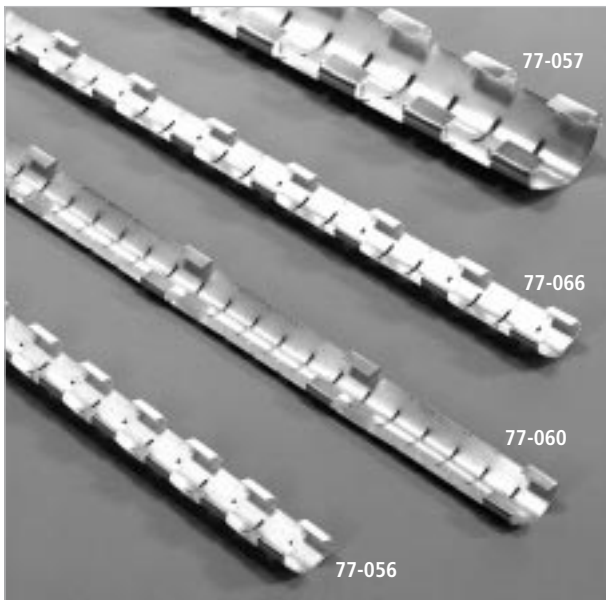
FIGURE 1: REPEATING FINGER PATTERN
