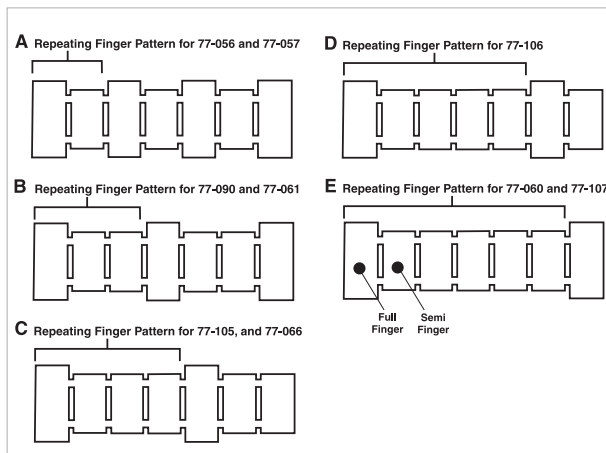
FIGURE 1: REPEATING FINGER PATTERN
