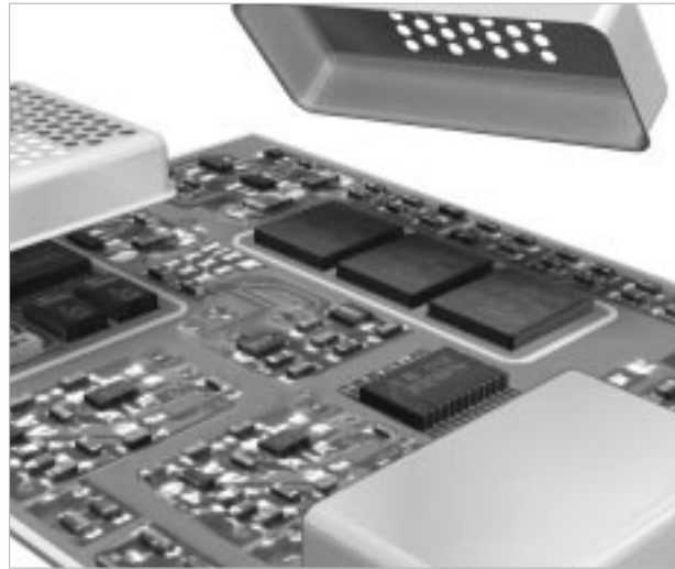
PRINTED CIRCUIT BOARD RADIATED TEST PER PDA-PRO-027 REV. A FOR DRAWN CAN SHIELD W/SOLDER VENTS VS. STANDARD CAN SHIELD
